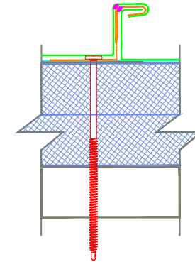
CROSS SECTION 90° SEAMING
