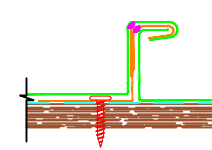
CROSS SECTION 90° SEAMING
